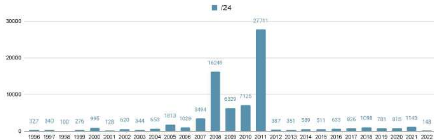
IPv4 Delegated /24
