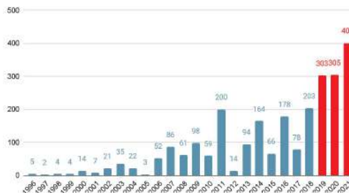
ASN Delegated
