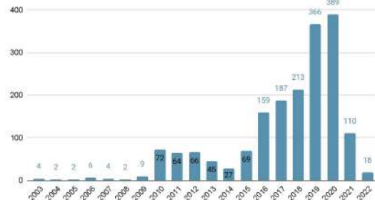
IPv6 Delegated /32
